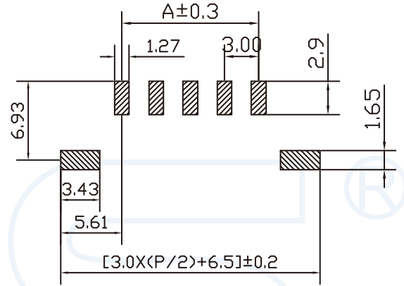
PCB LAYOUT:COMPONENT SIDE
